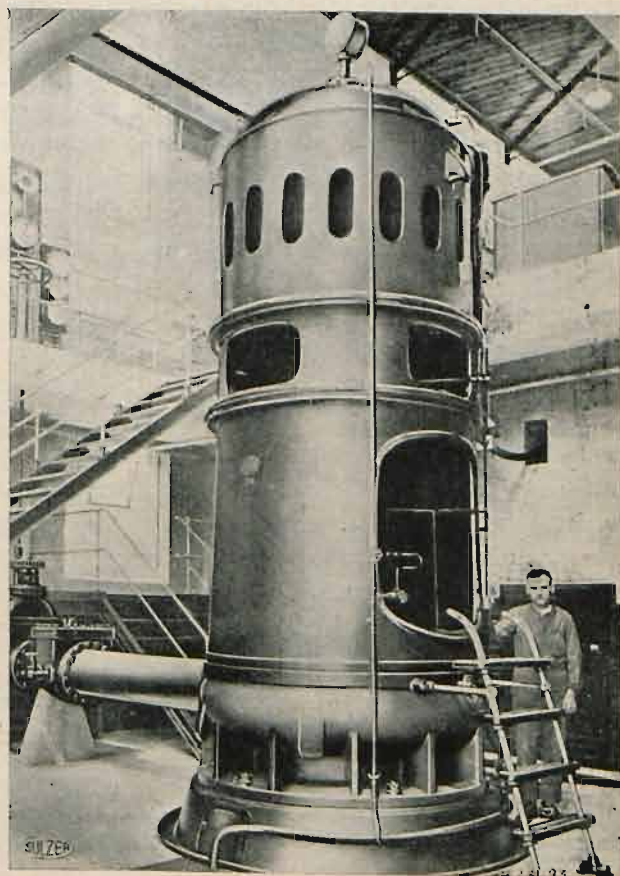
Rys. 12. South Staffordshire Waterworks Prestwold, Anglja, 158 l/sek. — 240 m — 663 HP.
